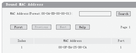
Figure 6-33 Bound MAC Address
